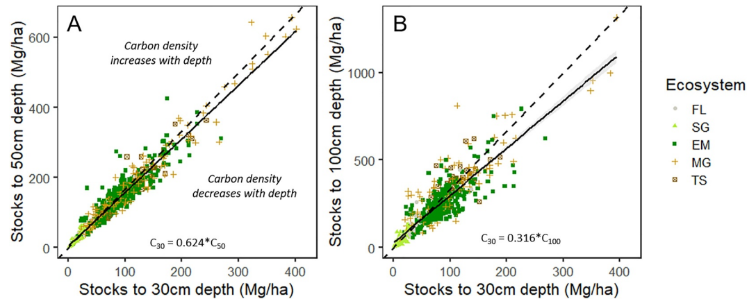
Figure 3. Correlation between sediment carbon stocks estimated to 30 cm depth versus (a) 50 cm depth and (b) 100 cm depth for all blue carbon ecosystems. Dashed lines show the null relationship expected between shallower and deeper stock estimates if carbon density were exactly uniform with depth. Solid lines and equations show actual relationships. Points below the dashed lines are cores in which carbon density decreased with depth (e.g., 30 cm stocks overestimate deeper stocks estimates), while points above the dashed lines are cores where carbon density increased with depth.
