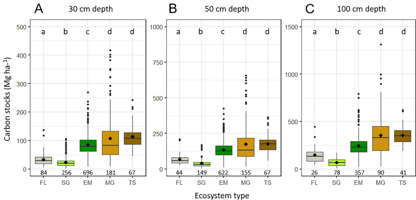
Figure 2. Sediment carbon stocks to (a) 30, (b) 50, and (c) 100 cm depth for five blue carbon ecosystems along the Pacific coast of North America. FL = tideflat; SG = seagrass; EM = marsh; MG = mangrove; TS = tidal swamp. Boxplots in this and subsequent figures show the median (horizontal line), mean (filled diamond), 25% and 75% of the data distribution (top and bottom of boxes), 1.5 times the interquartile range (whiskers), and outliers (dots). Ecosystem types sharing the same letters were not significantly different. Numbers below boxplots indicate sample sizes. Note different y-axis scales across panels.
