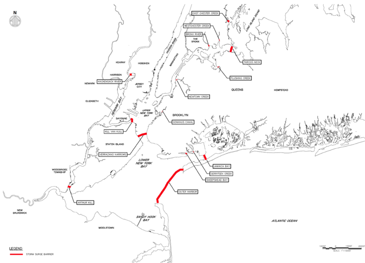
Figure 1: Map of conceptual storm surge barrier locations
