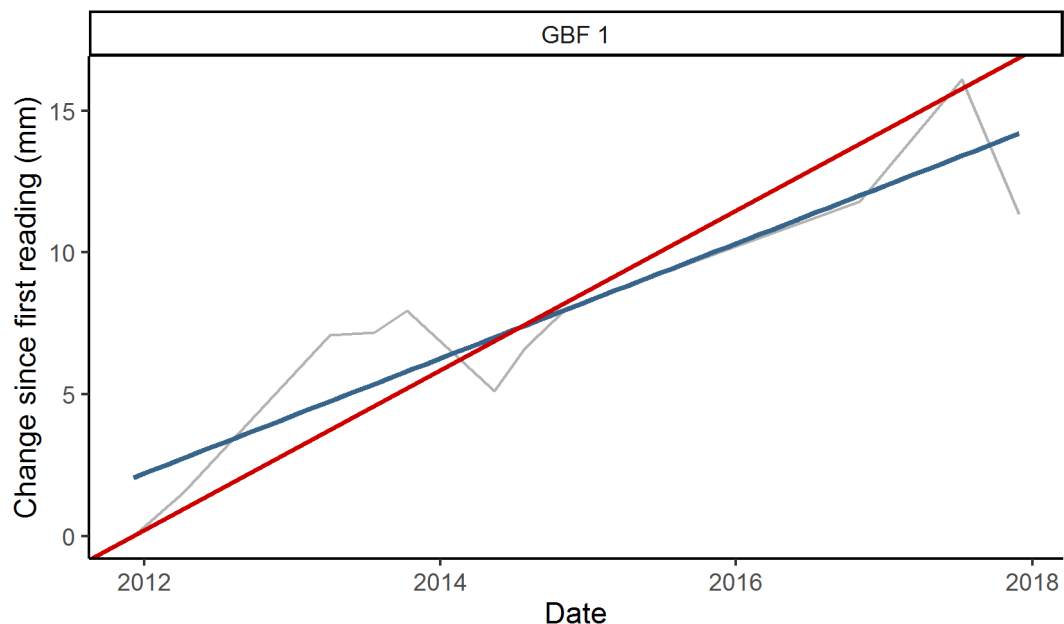
Figure 7. Average marsh surface height at one SET over time, as compared to the first reading. Gray line represents the data; the solid blue line is a linear regression of the data; the red line shows the rate of sea level change.
